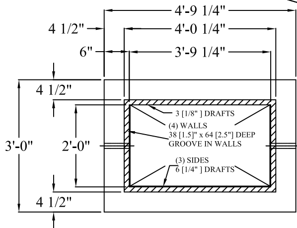
PLAN 24" X 45 1/4" TYPE S INLET TOP 39 1/2" X 57 1/4" X 18"
